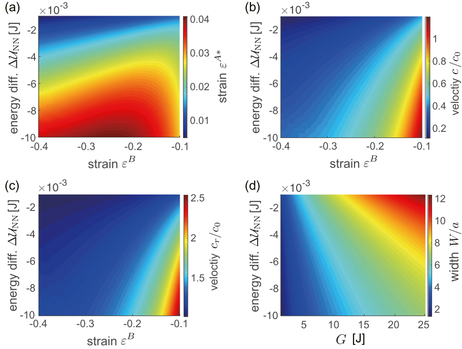
Fig. 6. (a) Evolution of \varepsilon^{A*} as a function of \varepsilon^B and \Delta\mathcal{L}_{NN} as predicted by Eq. (27). (b) Evolution of c/c_0 as a function of \varepsilon^B and \Delta\mathcal{L}_{NN} as predicted by Eq. (27). (c) Evolution of c_r/c_0 as a function of \varepsilon^B and \Delta\mathcal{L}_{NN} as predicted by Eq. (38). (d) Evolution of W/a as a function of G and \Delta\mathcal{L}_{NN} as predicted by Eq. (30).
